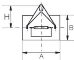
Ventosa a 1 piastra Single suction pad
