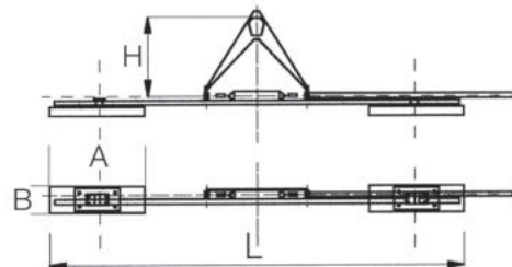
Ventosa a 2 piastre Two suction pads
