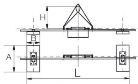
Ventosa a 2 piastre Two suction pads
